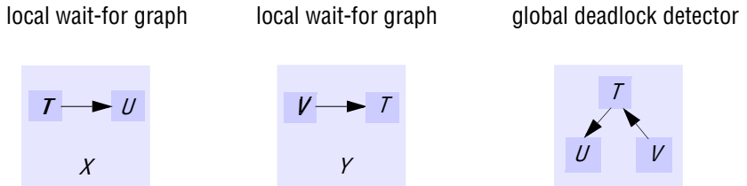
Figure 17.14 Local and global wait-for graphs
